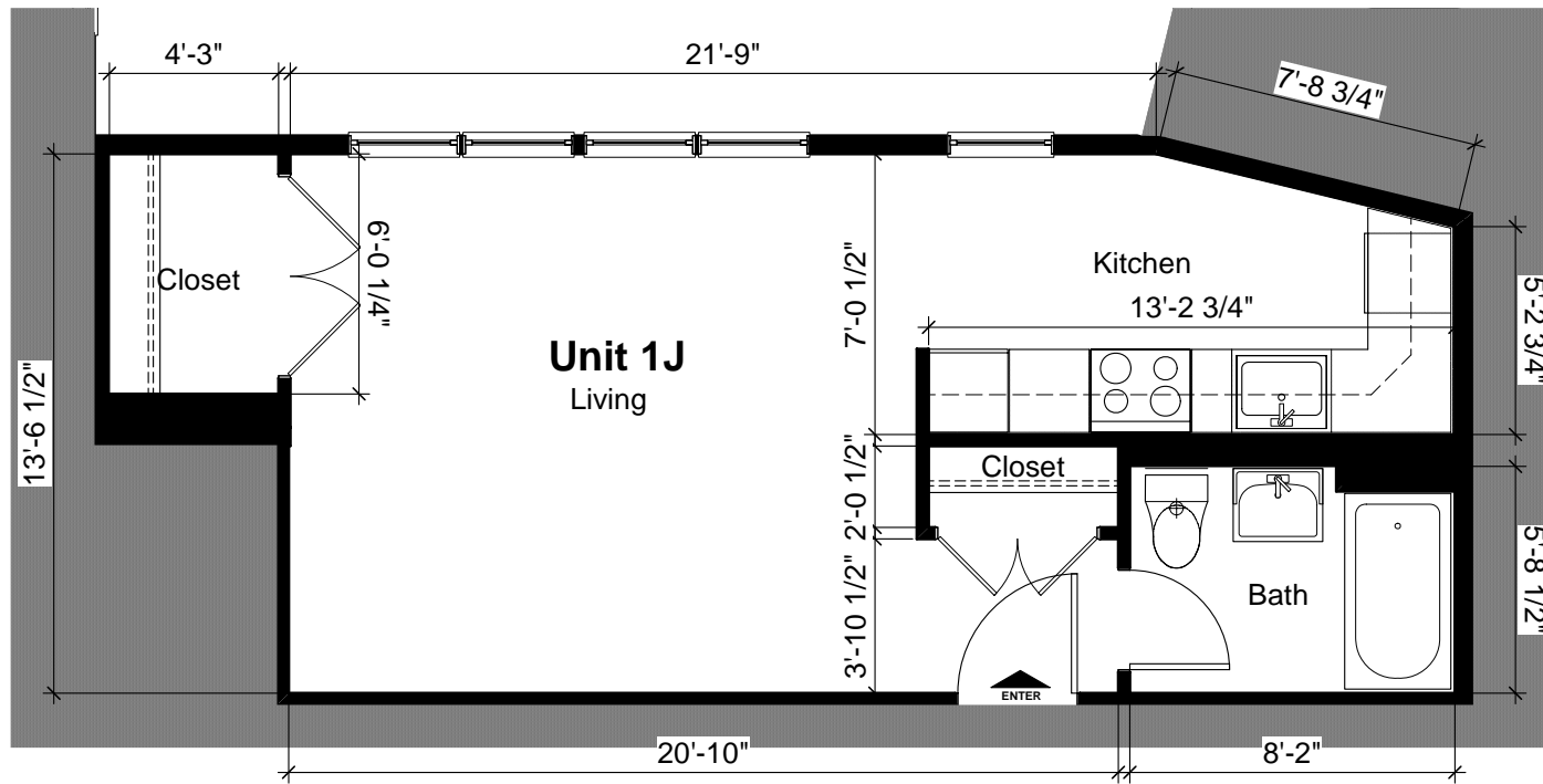
1 Unit J, 1st Floor 1J Scale: 3/16" = 1'-0" Unit Area = 424 sqft
